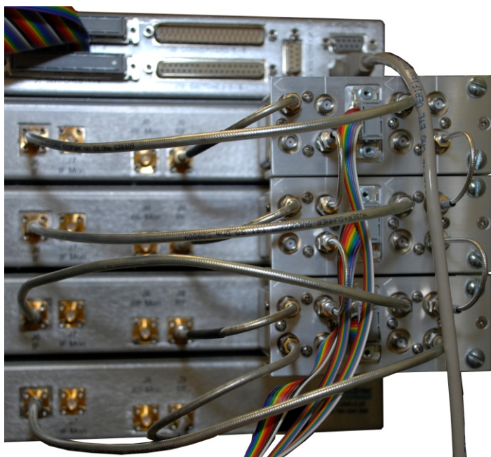
Typical 1:3 Redundant system Rear view with RNR controller, and three RSM-S50/S50 switch modules and four converters.
